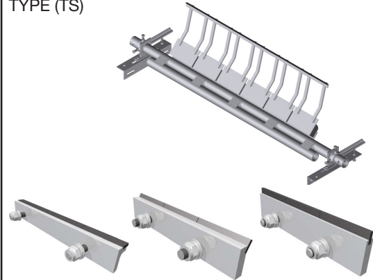
Reversible Belt Cleaner with Rubber & Tungsten Carbide Blade
